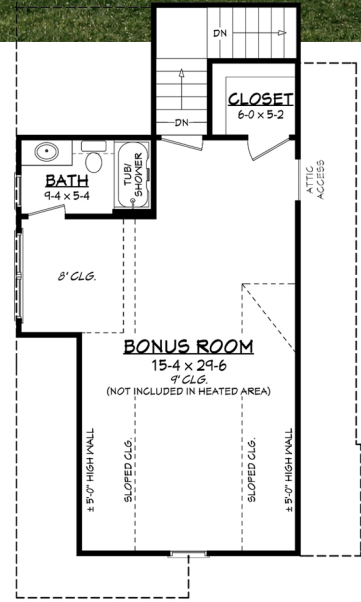
Bonus Floor Plan
