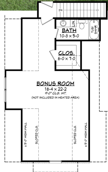
Bonus Floor Plan Square footage does not include bonus room.
