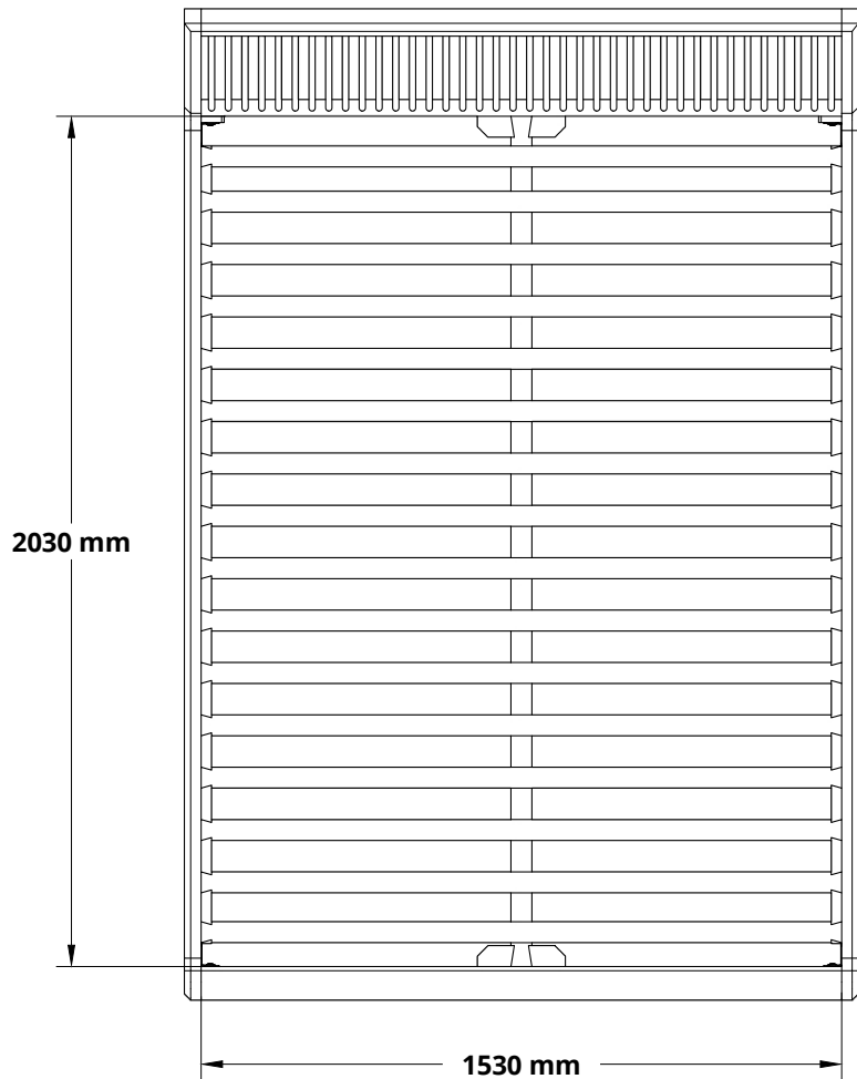
TOP VIEW
