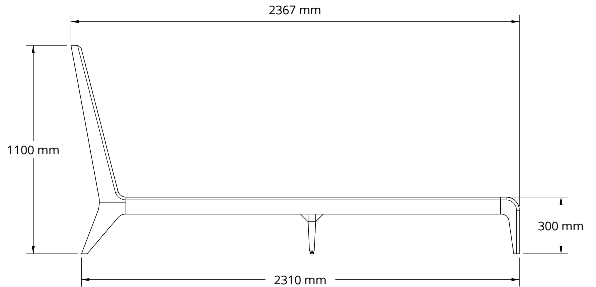
SIDE VIEW
