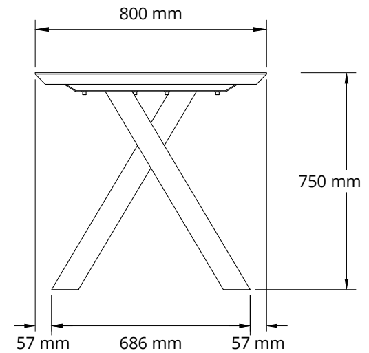
TAMPAK SAMPIING
