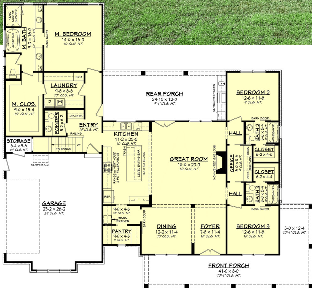
Floor Plan
