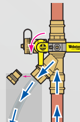
Flushing w/ Reverse Flow
