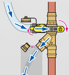
Flushing w/ Fresh Water
