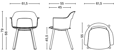
LAYOUT ARMCHAIR 221 Width 61,5 cm Depth 55 cm Height 79 cm Seat height 45,5 cm Armrest height 66 cm Weight 7,85 kg
