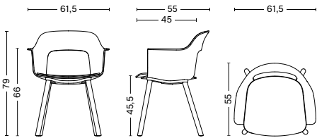
LAYOUT ARMCHAIR 222 Width 61,5 cm Depth 55 cm Height 79 cm Seat height 45,5 cm Armrest height 66 cm Weight 7,55 kg
