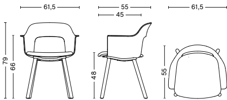
LAYOUT ARMCHAIR 223 Width 61,5 cm Depth 55 cm Height 79 cm Seat height 48 cm Armrest height 66 cm Weight 8,45 kg
