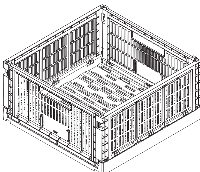
LARGE SQUARE W42 x L42 x H21,5 cm
