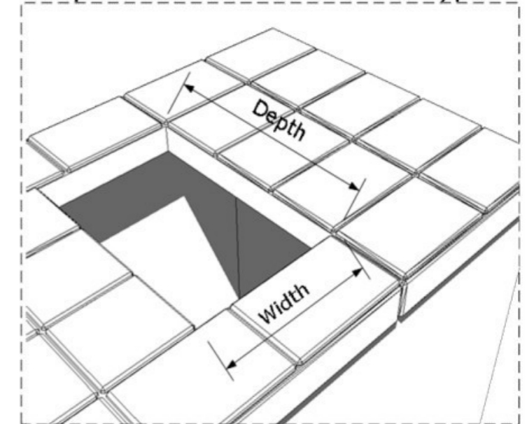
Drop-In Side Burner Cut-out Type
