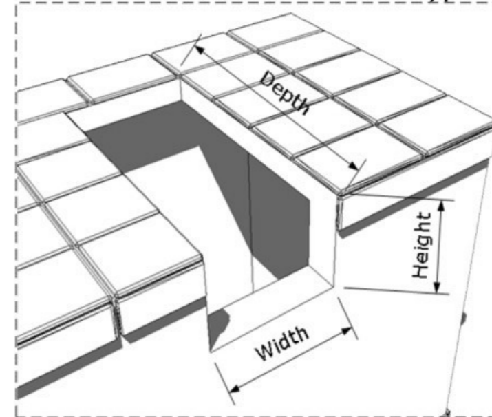
Slide-In Side Burner Cut-out Type
