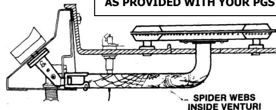
Spider webs inside venturi
