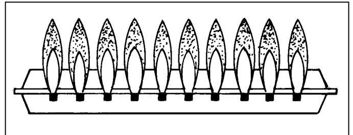
NORMAL HARD FLAMES Slightly out of adjustment burner
