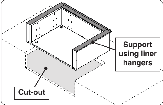
Fig. 1-1 Installation orientation
