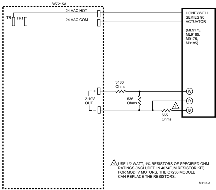
Fig. 1. W7215A used with Honeywell Series 90 Actuator.
