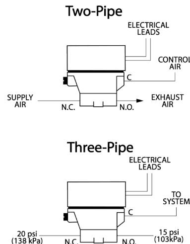
Fig. 1. Application diagram.
