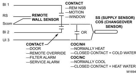
Fig. 4. Remote Inputs
