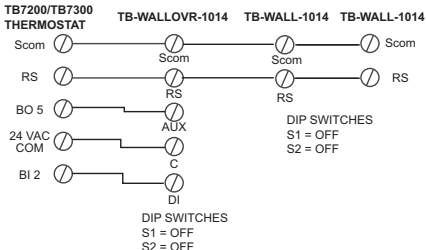
Fig. 7. Wiring examples of three remote wall mounted room sensors for averaging applications
