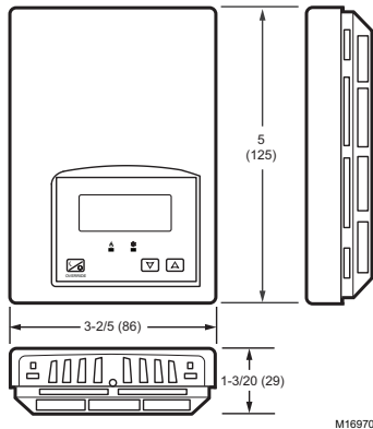
Fig. 10. Thermostat dimensions in inches (mm)
