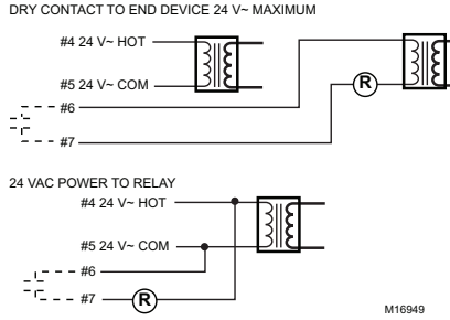
Fig. 8. Auxiliary Inputs
