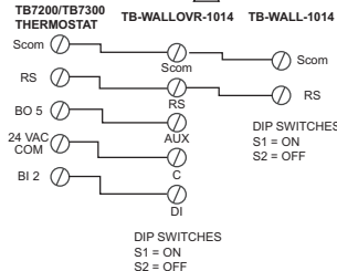
Fig. 6. Wiring examples of two remote wall mounted room sensors for averaging applications
