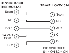
Fig. 5. Wiring example of single remote wall mounted room sensor
