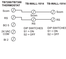
Fig. 6. Wiring examples of two remote wall mounted room sensors for averaging applications
