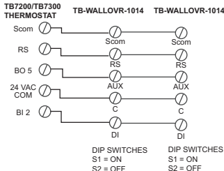
Fig. 6. Wiring examples of two remote wall mounted room sensors for averaging applications
