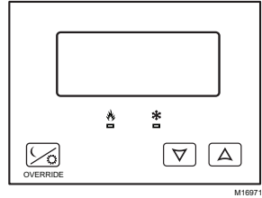
Fig. 9. Zoning model thermostat buttons and display
