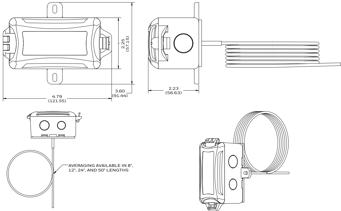
Fig. 4. C7021R, C7023R, C7041R dimensions in in. (mm).
