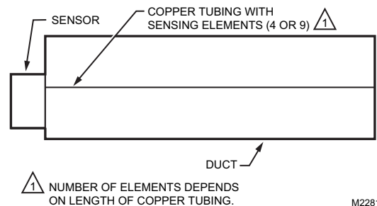
Fig. 6. Duct cross section showing method of installing C7021R, C7023R, C7041R in a multizone system.
