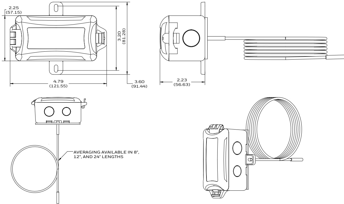
Fig. 1. C7021J, C7023J, C7031J, C7041J dimensions in in. (mm).
