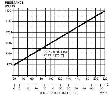
Fig. 5. C7130B resistance vs. temperature performance characteristics.
