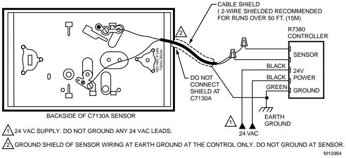
Fig. 3. General wiring hookup for C7130A sensor to R7380 Controller.
