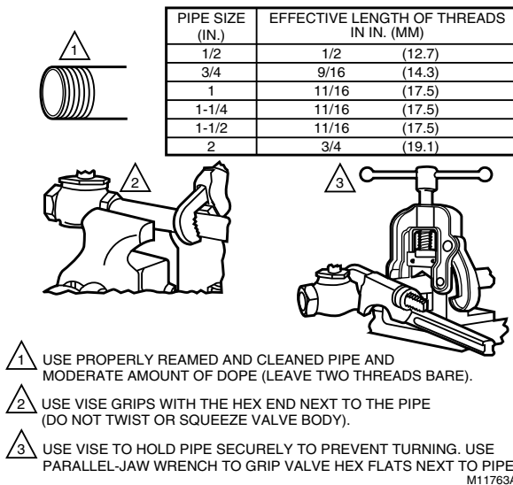
Fig. 4. Installing valves with threaded connections.
