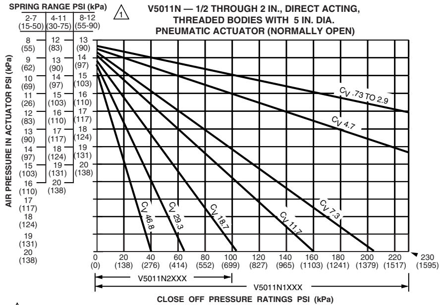
Fig. 3. Close-off ratings at various control air pressures for V5011N Valves and MP953 Pneumatic Actuators.
