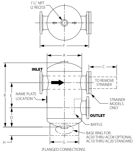
(FLANGED CONNECTIONS)
