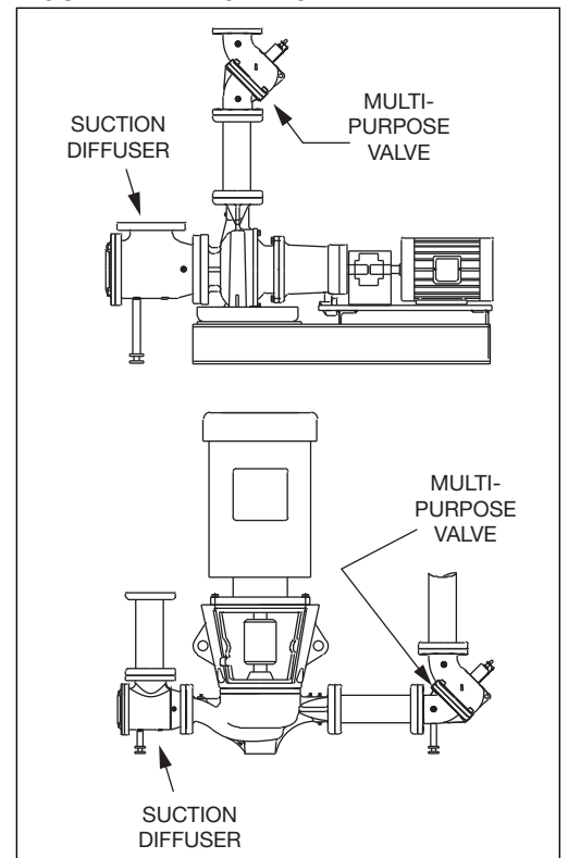
FIGURE 1: PIPING DIAGRAM
