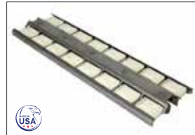
VIKCT2 Stainless Steel Ceramic Briquette Tray & Briquettes 18-1/8" x 5-7/16" Use with: CG114SS
