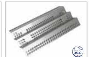
AOGHP2 Stainless Steel Heat Plate 15-1/2" x 8-1/4"
