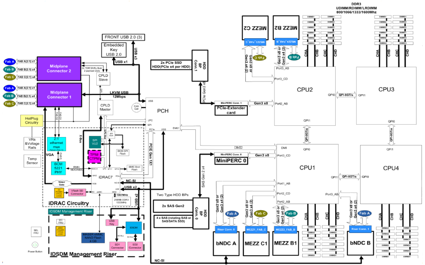
Figure 9. M820 system board block diagram
