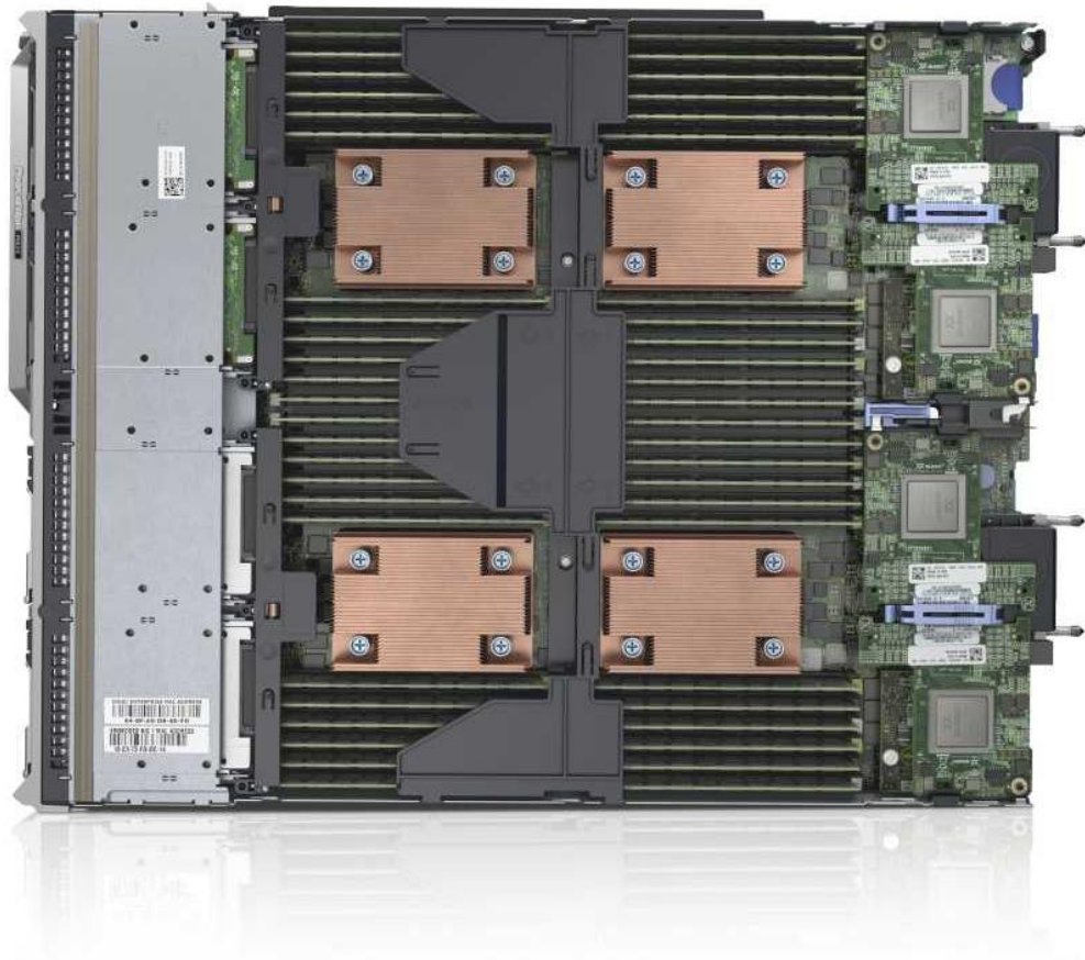
Figure 3. M820 internal module view
