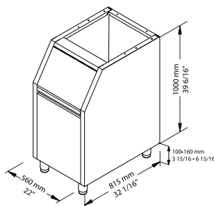
Adjustable feet 3 15/16" – 6 15/16"
