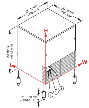
Adjustable feet 4 5/16" – 5 14/16"
