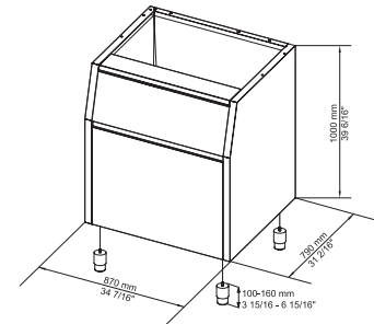
Adjustable feet 3 15/16" – 6 15/16"
