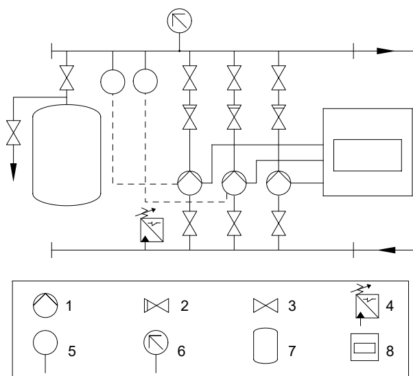
Schematic drawing of systems with three pumps
