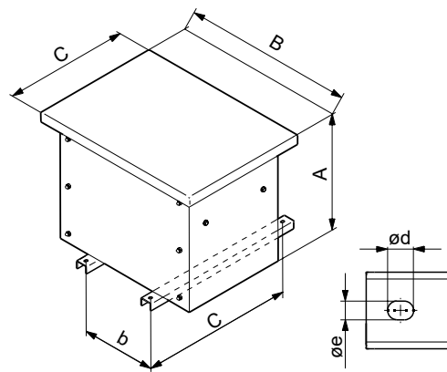
Floor mounting
