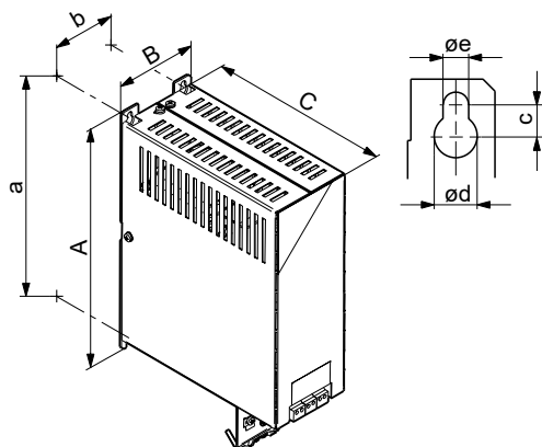
Wall mounting
