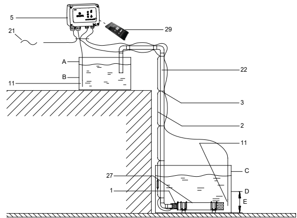
Pumping from one tank to another
