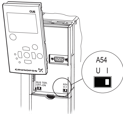
Setting contact A54 to current signal "I"
