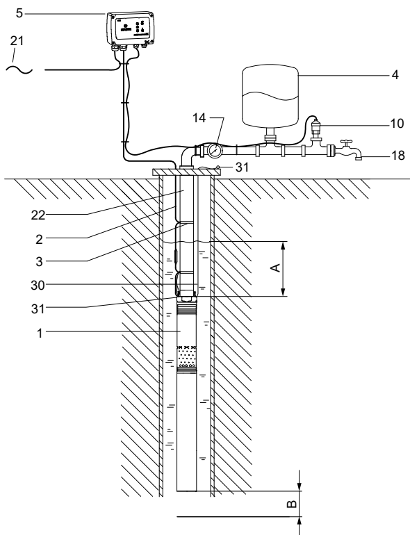
Application example: Constant-pressure control with CU 302 - residential water supply
