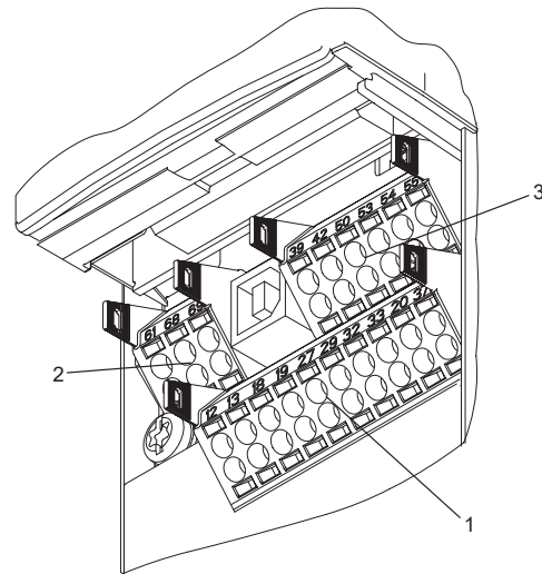
Signal terminals
