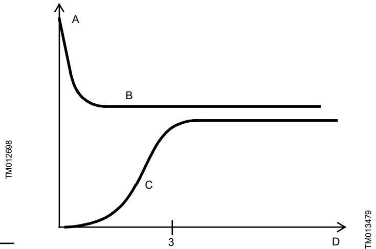
Soft-start feature
