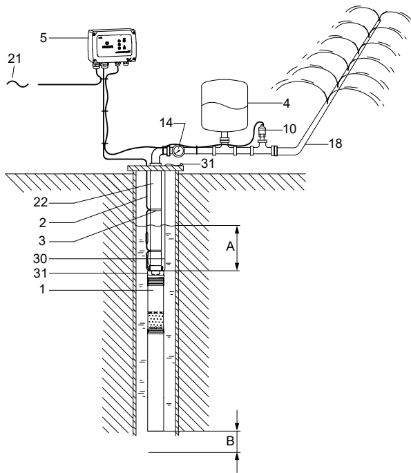
Application example: Constant-pressure control with CU 302 - irrigation
