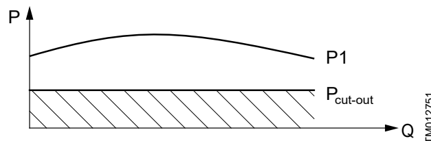
P_{\text{cut-out}} curve
