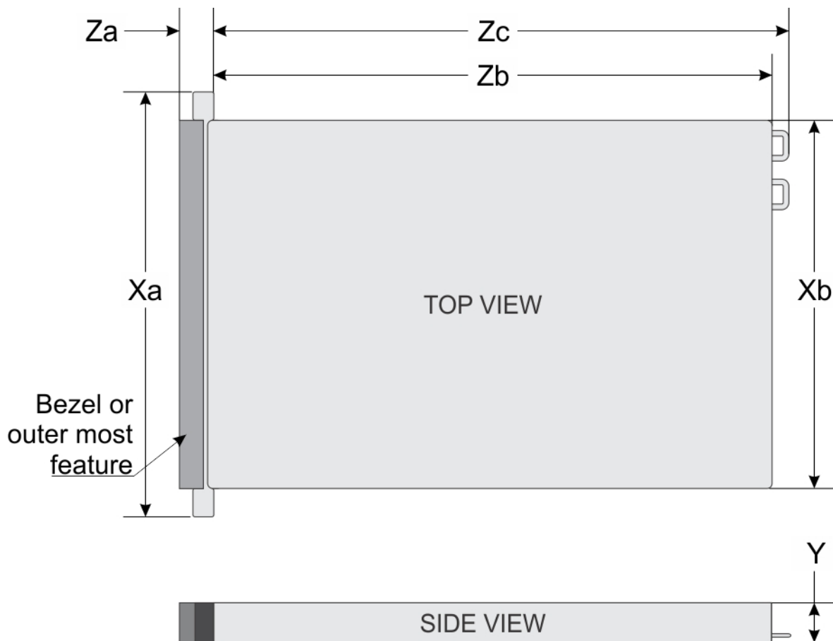
Figure 18. PowerEdge R550 chassis dimensions
