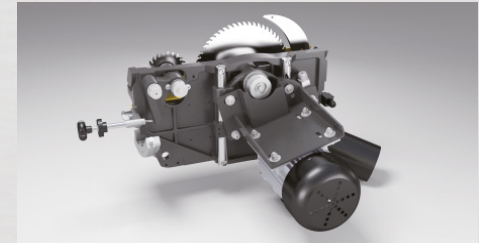
The cast iron saw unit provides extra support and stability for reduce vibration.
