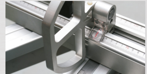
Large section profile cross cutting fence with reversible fence stops.
