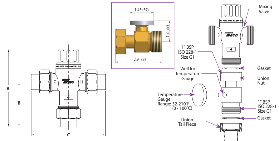
5120 Series Mixing Valve Dimensions Dimensions for reference only
