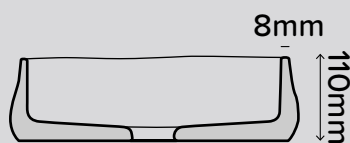
SECTION VIEW
