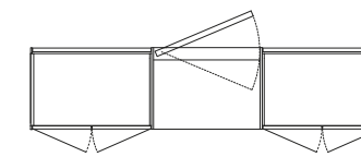
porta singola, allineamento retro armadio - apertura dx single door, wardrobe back alignment - right opening
