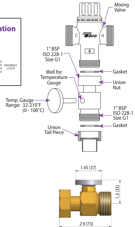
5000 Series Heating Only Mixing Valve Dimensions Dimensions for reference only
