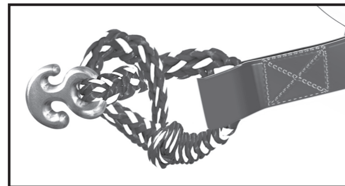
2: Loop the Aluminum Connector down around and through the bottom loop in diagram 1: and pull the Aluminum Connector through the loop. Note to pull until taut as shown below in 3:
