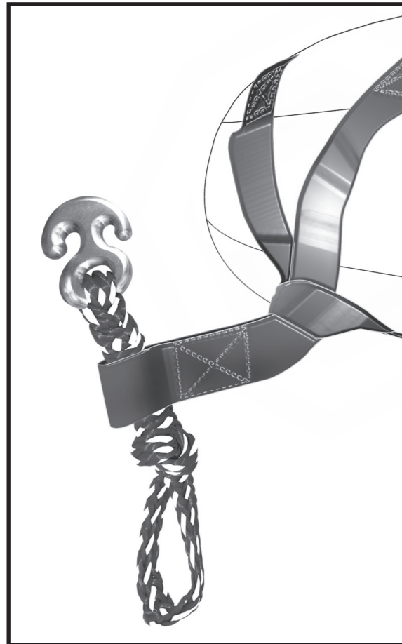
1: Locate the loop on the towable tow strap that is sewn to the towable. Put the 4K EZ Tow Aluminum Connector through the towable strap loop as shown above.
