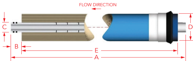
All TF – 1812 Residential Membrane Elements seal at a standard 2.00 inch – 2.05 inch I.D.
