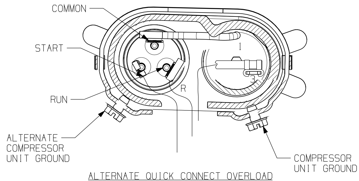
ALTERNATE B-B
