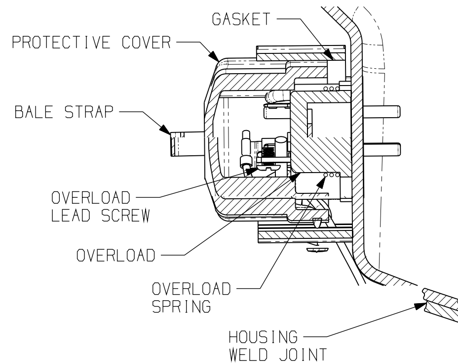
SECTION C-C
