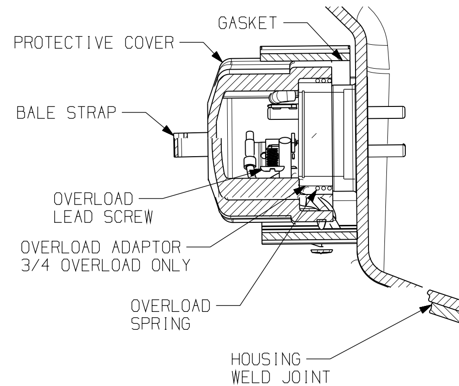
ALTERNATE C-C
