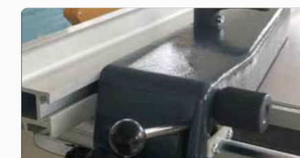
Reversible sawing fence that folds up the workbench when hands need to be freed to saw large boards.
