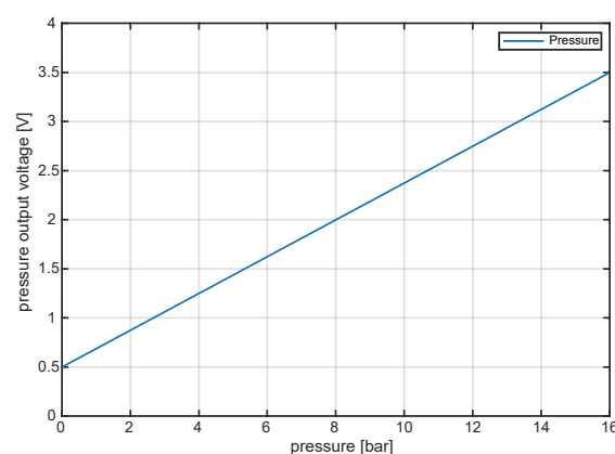
Pressure response in analogue mode
