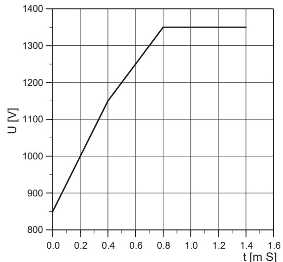
Maximum values for voltage peaks
