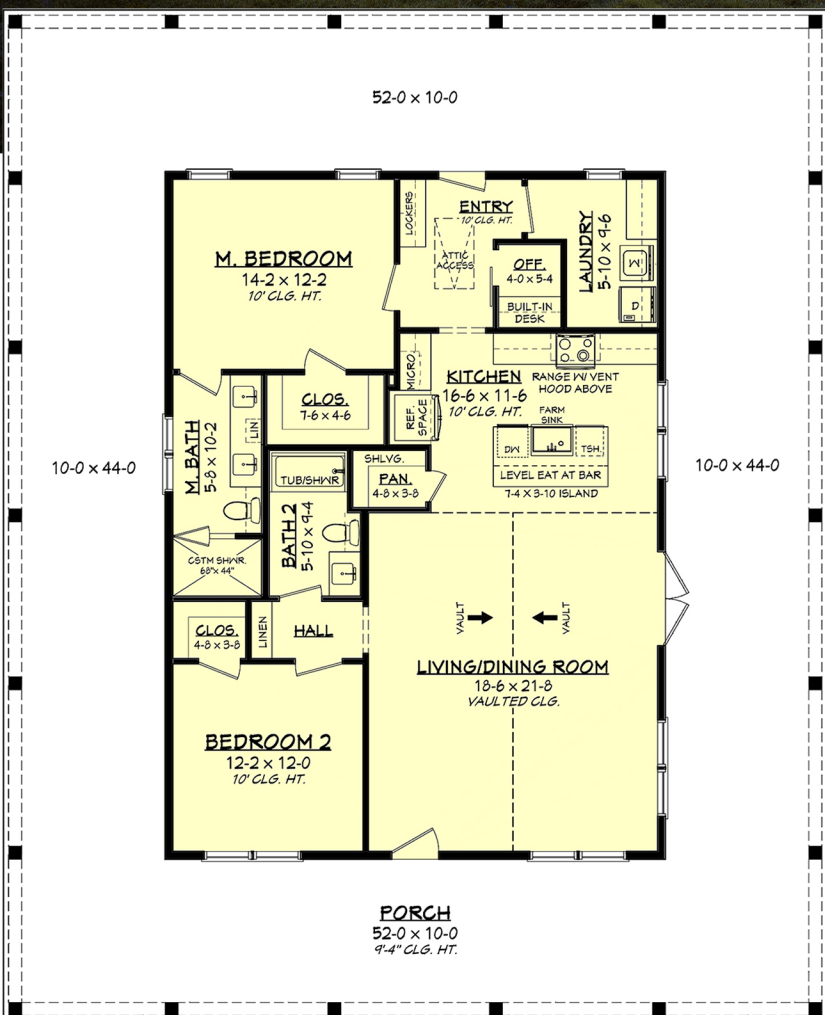
Floor Plan
