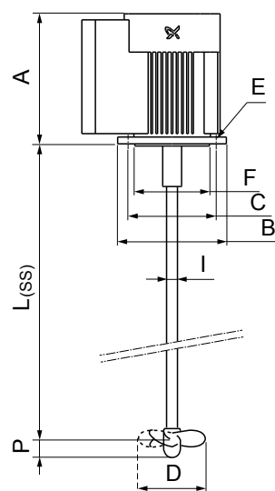
Fig. Electric stirrer, stainless steel version
