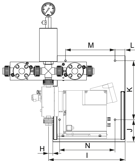
Fig. Preassembled accessories set in side view
