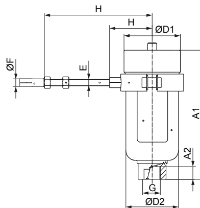
Fig. Pulsation damper DB, stainless steel version
