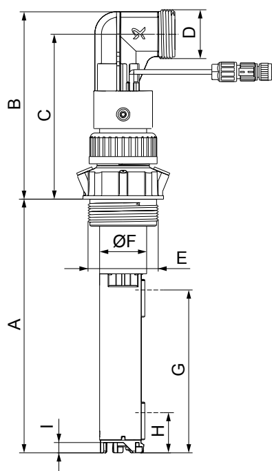
Fig. Rigid suction lance
