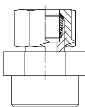
Fig. Pipe connection 10/12 mm
