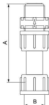
Fig. Dimensions of pressure valve PV
