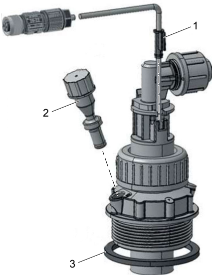
Fig. Emission protection kit
