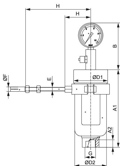
Fig. Pulsation damper DBG-H
