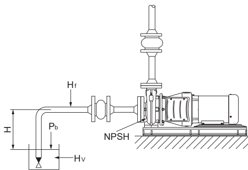
Suction lift with positive H
