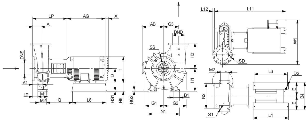
Dimensional drawing, mounting design B, tangential outlet
