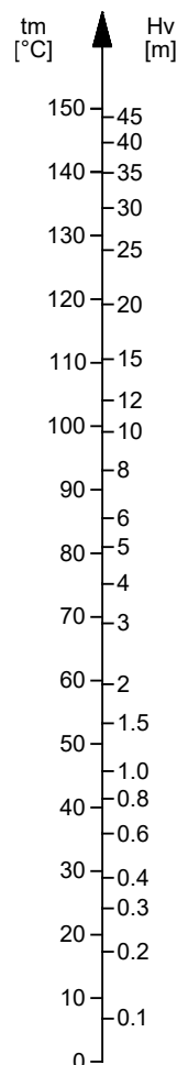
Relation between liquid temperature and vapor pressure
