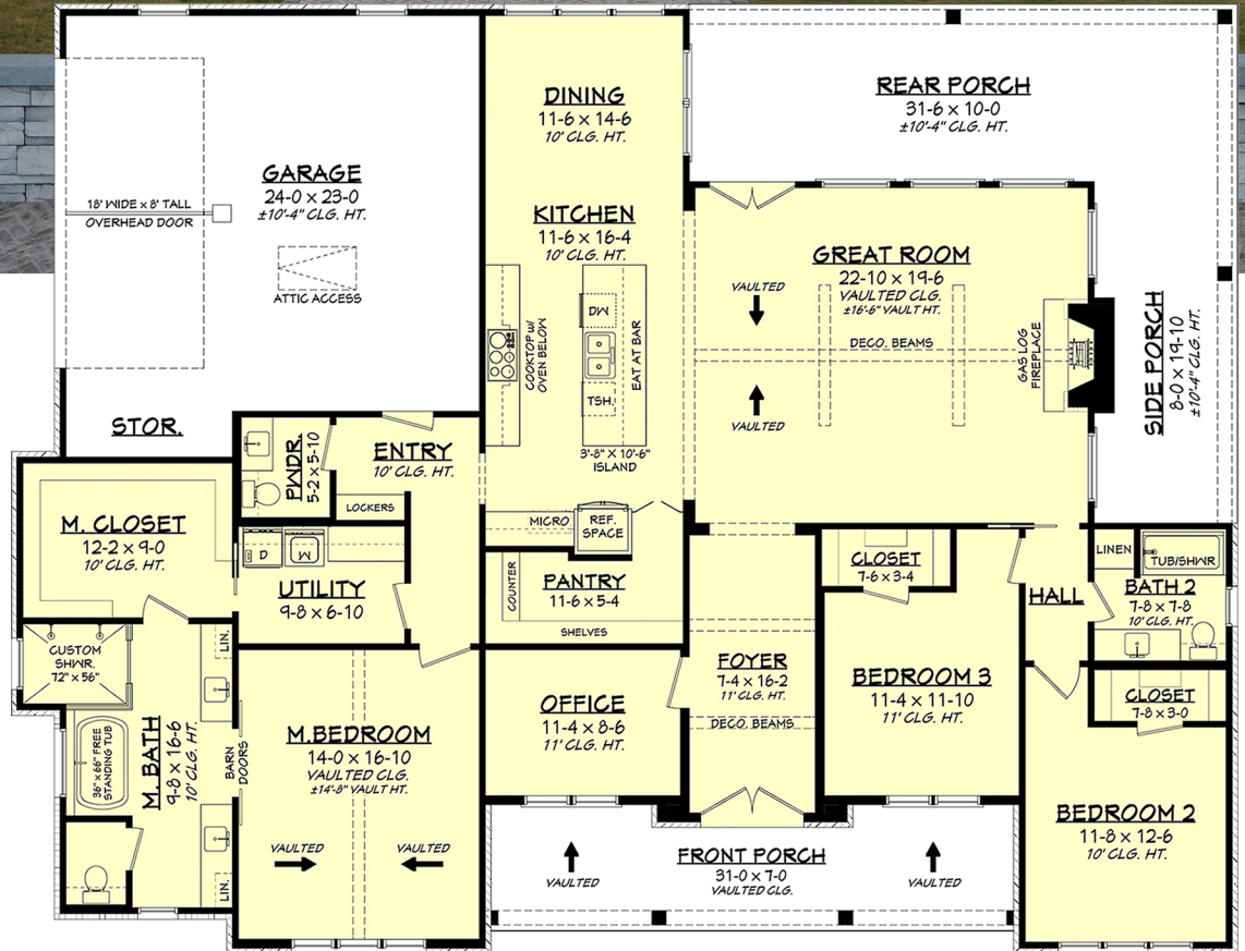
Floor Plan
