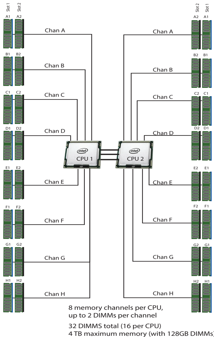
Figure 3 B200 M6 Memory Organization
