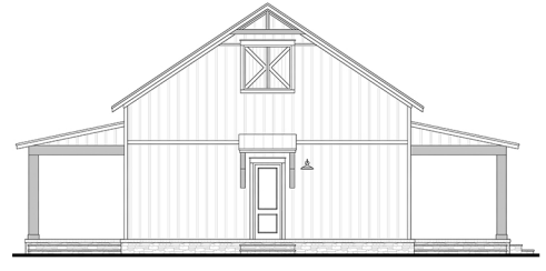
Rear Elevation
