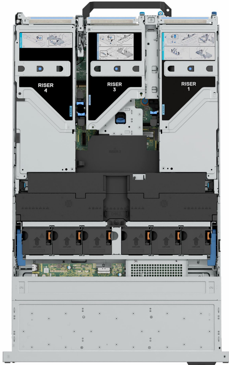
Figure 11. Inside the system with full length risers and GPU shroud
