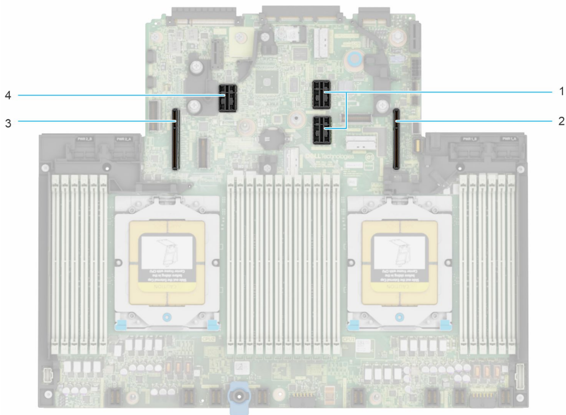
Figure 14. Expansion card riser slot connectors
