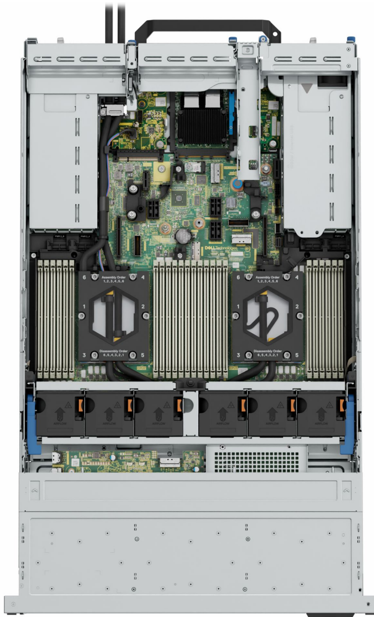
Figure 12. Inside the system with processor liquid cooling module
