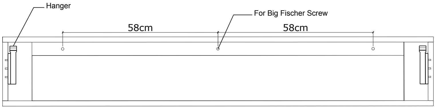
BACK VIEW
