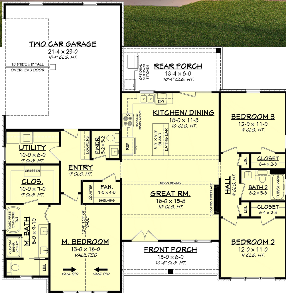
Floor Plan
