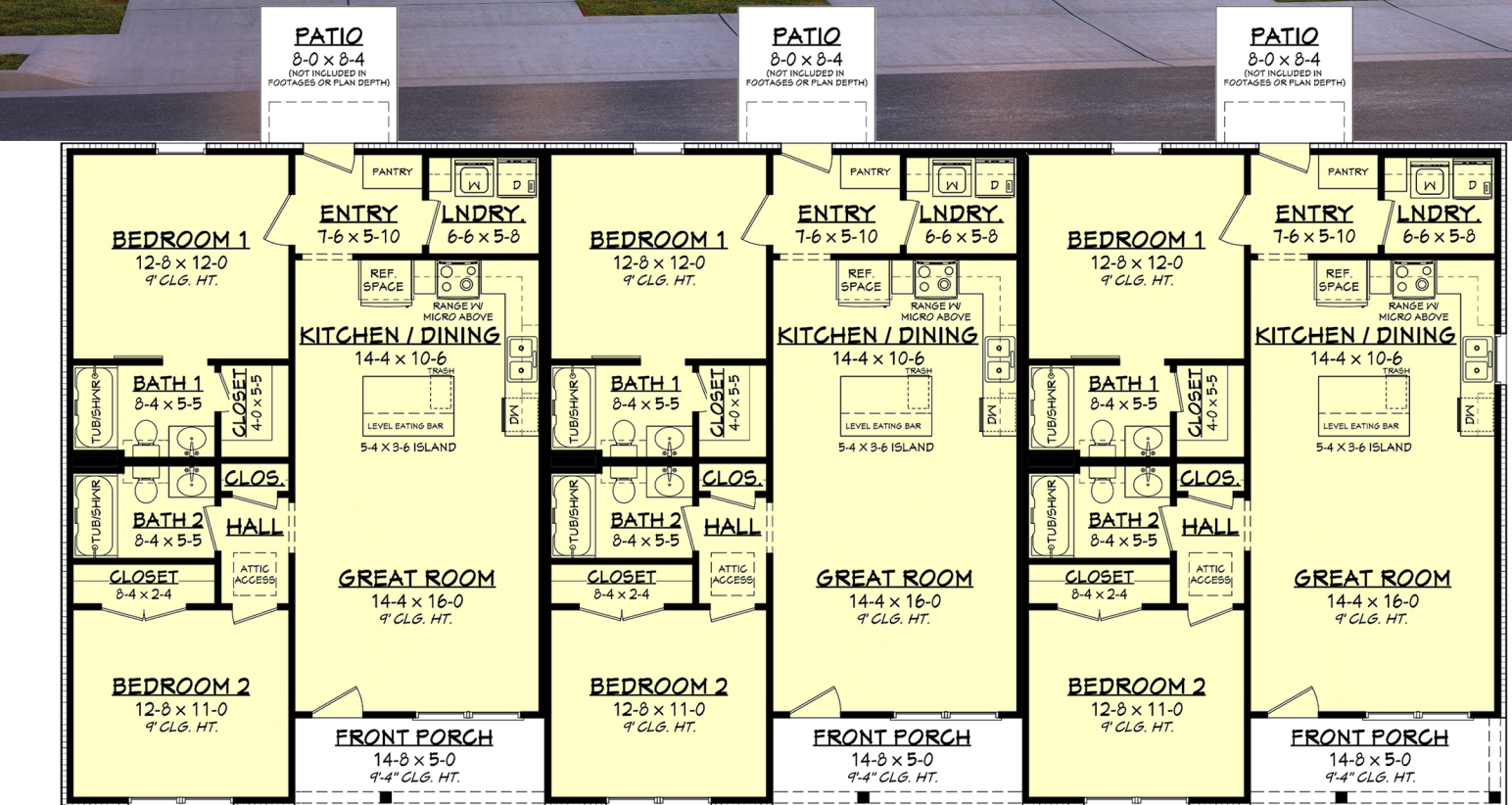
Floor Plan
