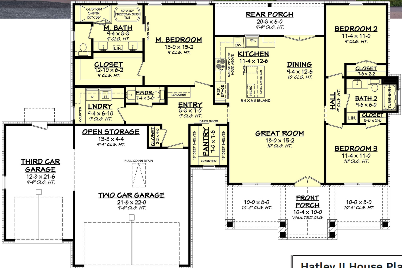
Floor Plan
