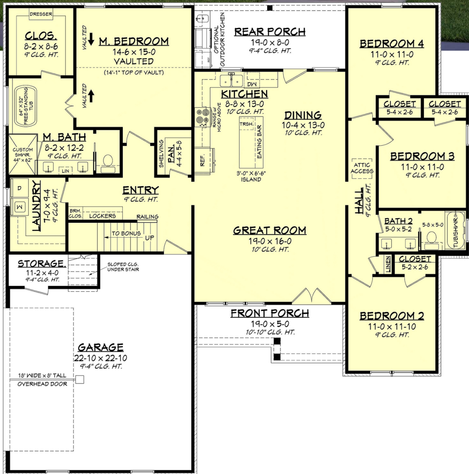
Floor Plan
