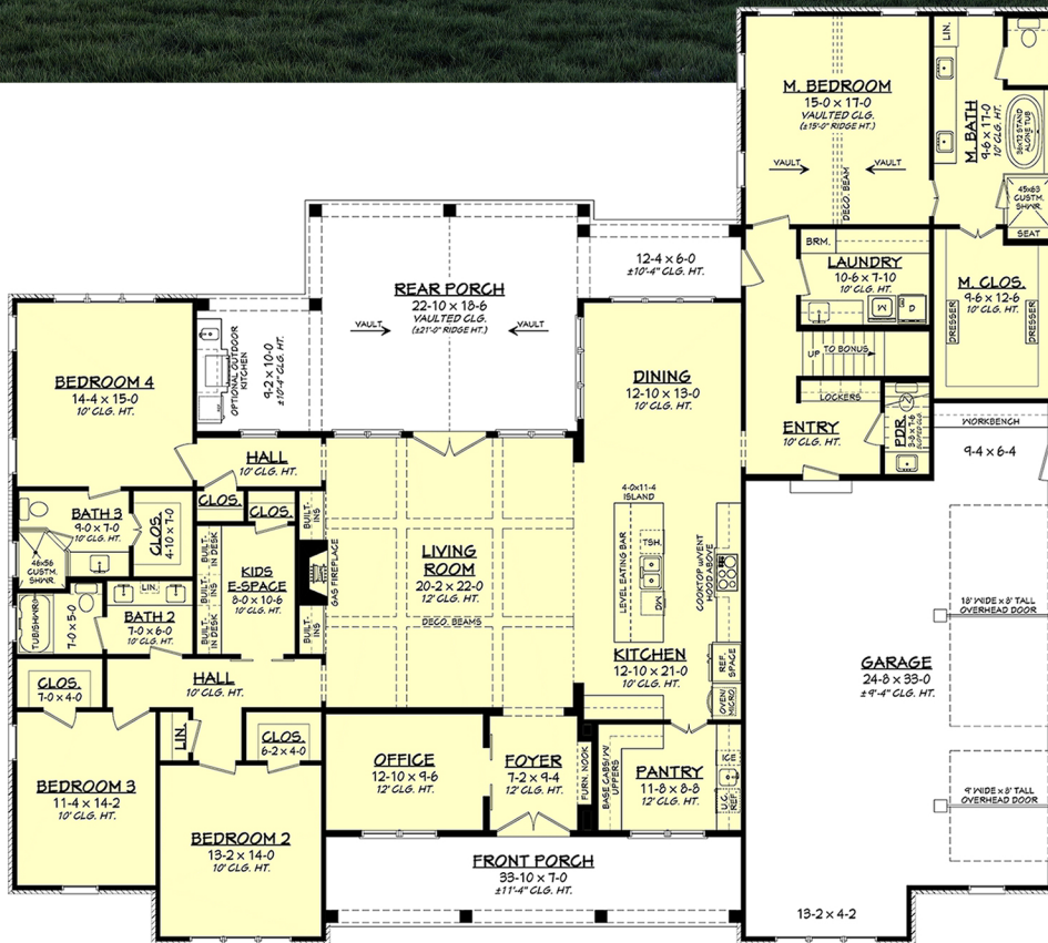
Floor Plan
